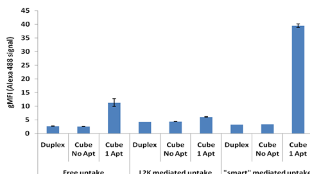
Figure 5. Uptake of siRNA duplex, cubes decorated with 3 Alexa-488 fluorescent probes, and cubes decorated with 3 Alexa-488 fluorescent probes and 1 Sgc8c aptamer, mediated by L2K or "smart" \beta -CD polymer in CEM cells.
